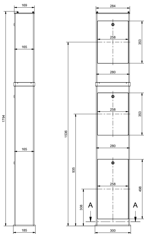
Housing MS 1800
