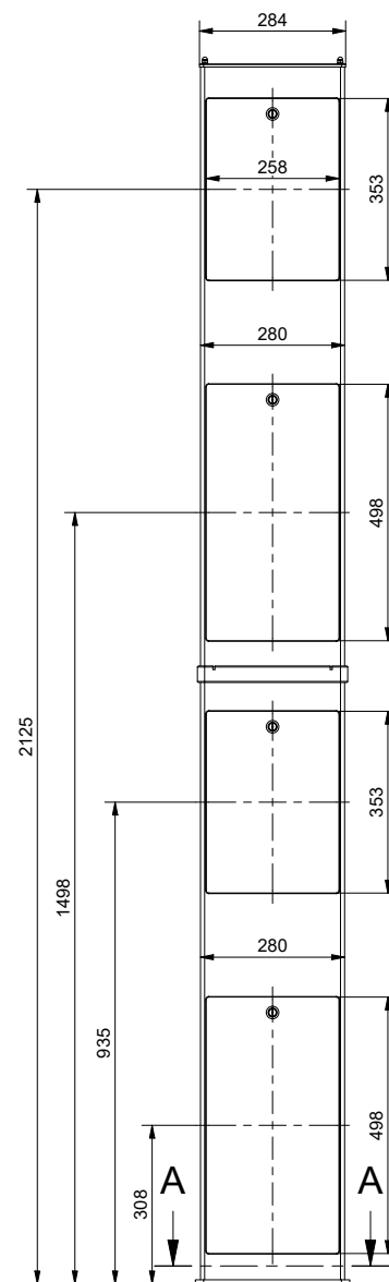
Housing MS 2400
